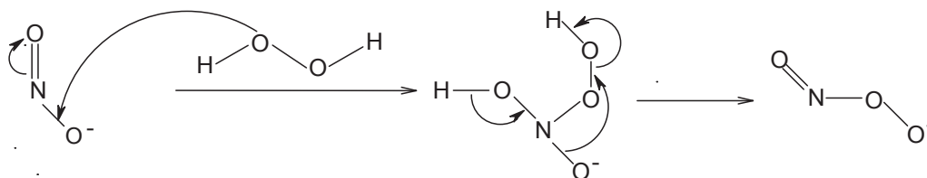
Figure 6. Baeyer-Villiger-like reaction scheme of peroxynitrite synthesis from sodium nitrite and acidified hydrogen peroxide.
