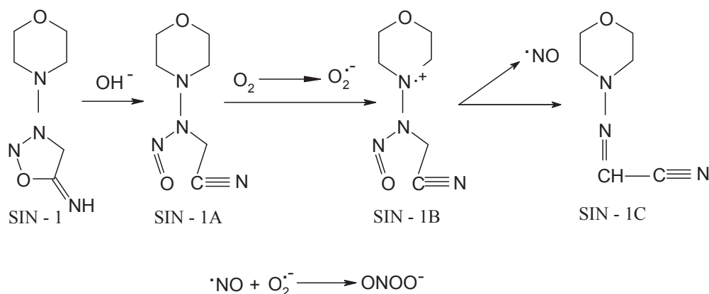
Figure 7. Peroxynitrite formation from SIN-1 (Hrabárová et al. 2007).
